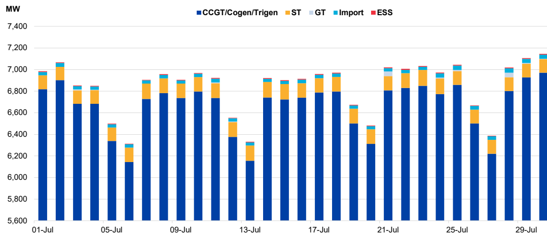
Figure 5: Generation by Type for This Month
