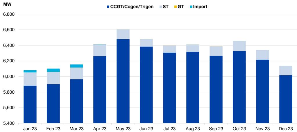
Figure 4: Average Generation by Type for Last 12 Months
