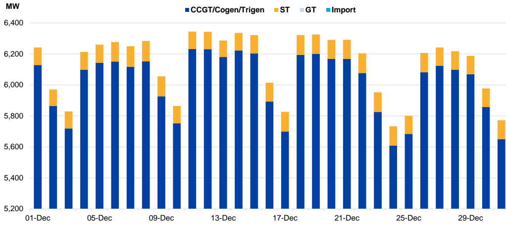
Figure 3: Average Generation by Type for This Month
