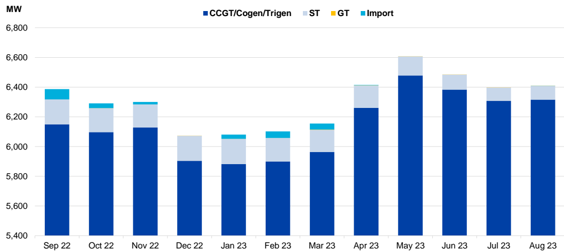
Figure 4: Average Generation by Type for Last 12 Months
