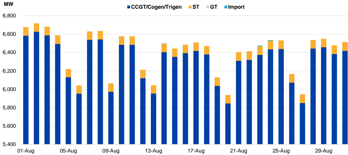
Figure 3: Average Generation by Type for This Month
